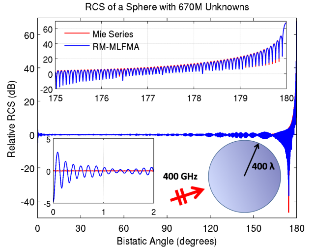
Fig. 4. RCS of a sphere with 670 million unknowns.
