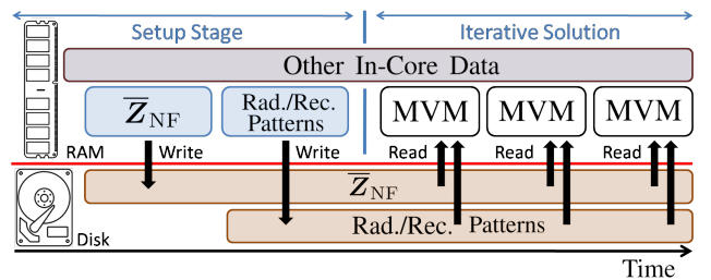
Fig. 1. Out-of-core method for MLFMA.
